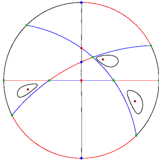
FIGURE 1. Phase portrait in the Poincaré disc of the cubic system (3.7).
