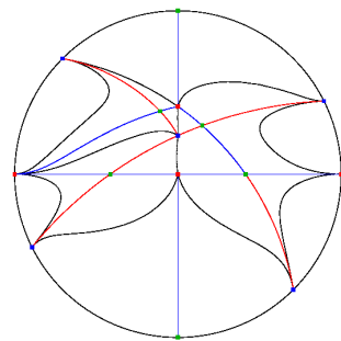
FIGURE 3. Phase portrait in the Poincaré disc of the cubic system (3.9).
